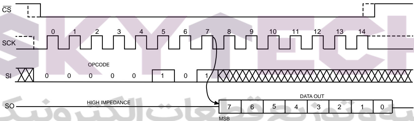
Figure 5. RDSR Timing
