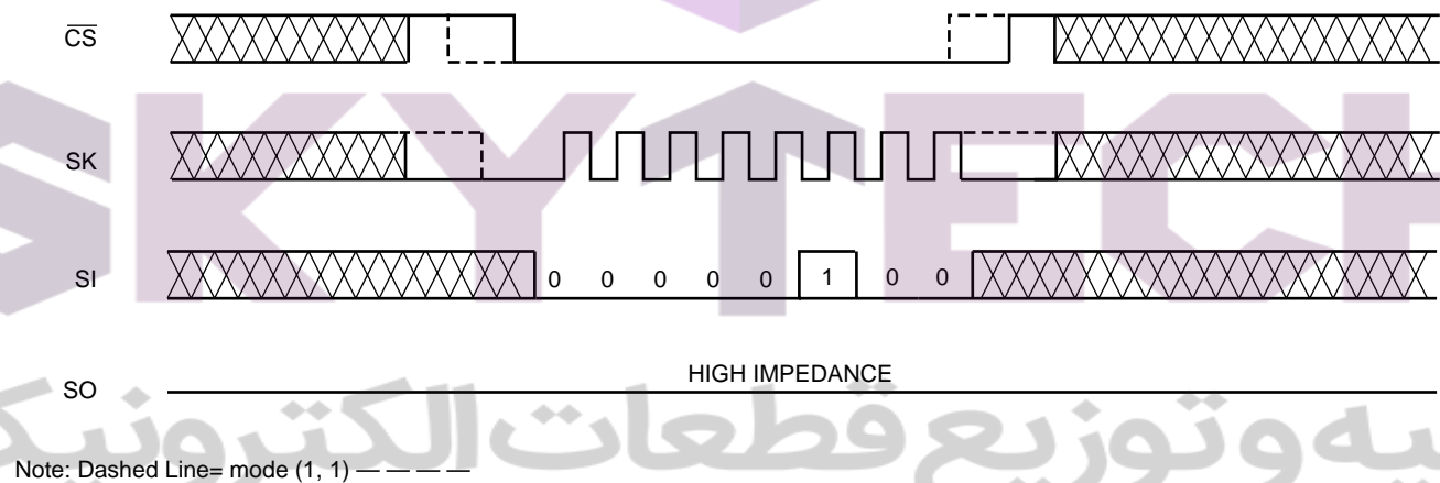
Figure 3. WRDI Instruction Timing
