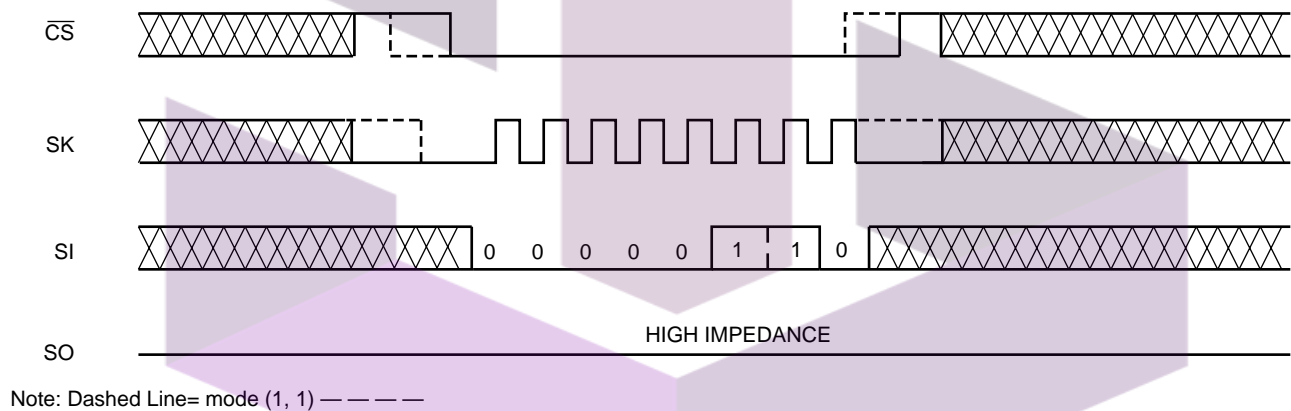
Figure 2. WREN Instruction Timing
